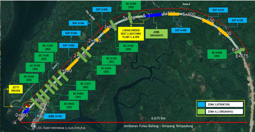
Plan of IKN Toll Road Section 5A Simpang Tempadung-Jembatan Pulau Balang
